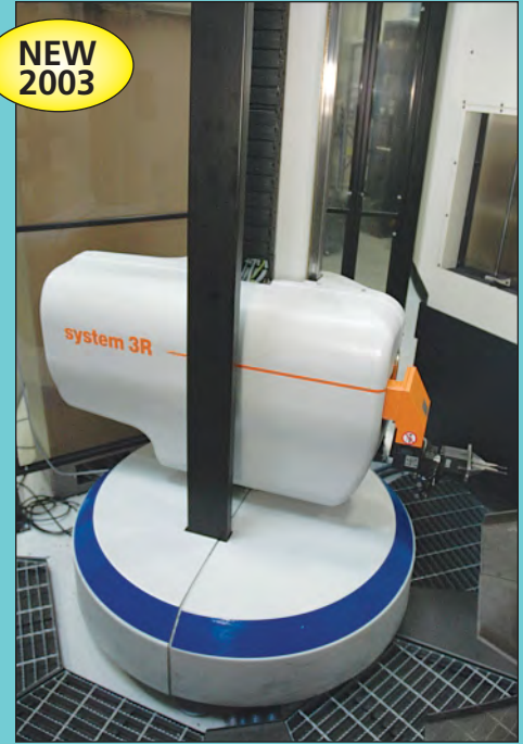
System 3R Workmaster Type K-50623 Automatic Tool Changer Robot
