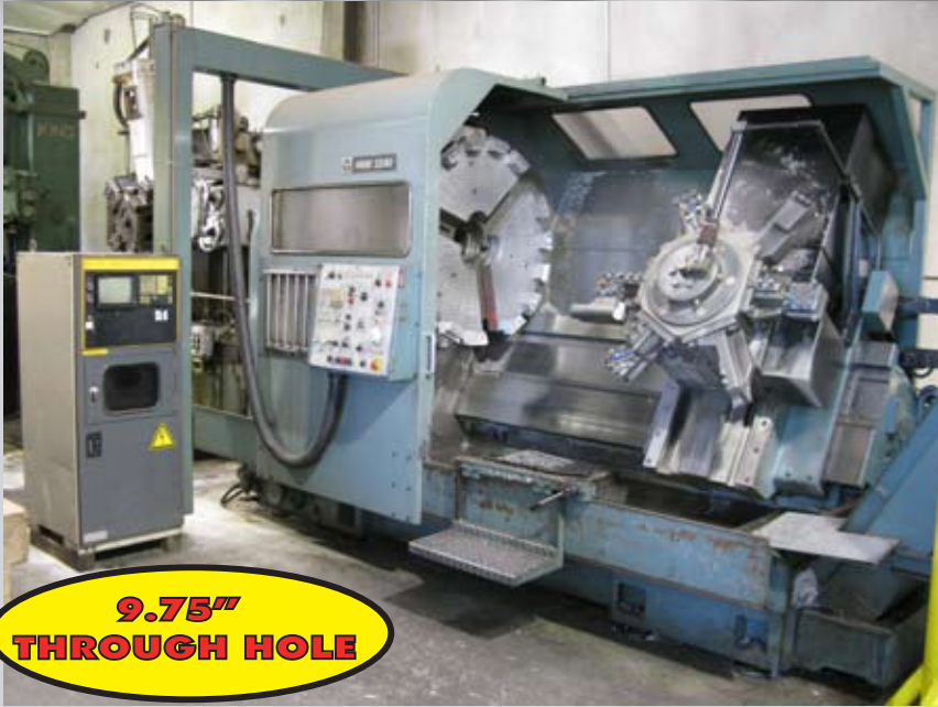
MORI SEIKI SL-8F CNC TURNING CENTER W/FANUC 11T, 36" CHUCK, 45" SWING.
